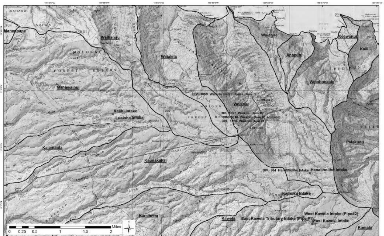
Figure 11. Molokai Properties' Molokai Water System diverts water from the surface water hydrologic units of Kawela, Kaunakakai, Waikolu, and Manawainui.
