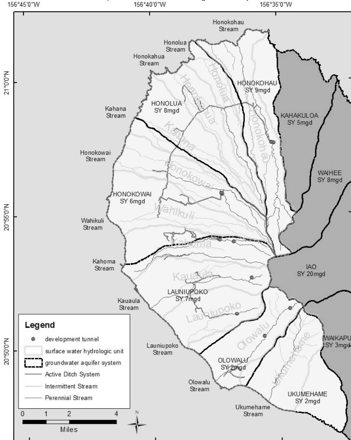
Figure 13. Lahaina Aquifer Sector Area. Ground Water Aquifer Systems Areas and their sustainable yields (SY) for the Lahaina Aquifer Sector with overlaying surface water hydrologic units and their perennial and intermittent streams with development tunnels and active irrigation ditch systems.
