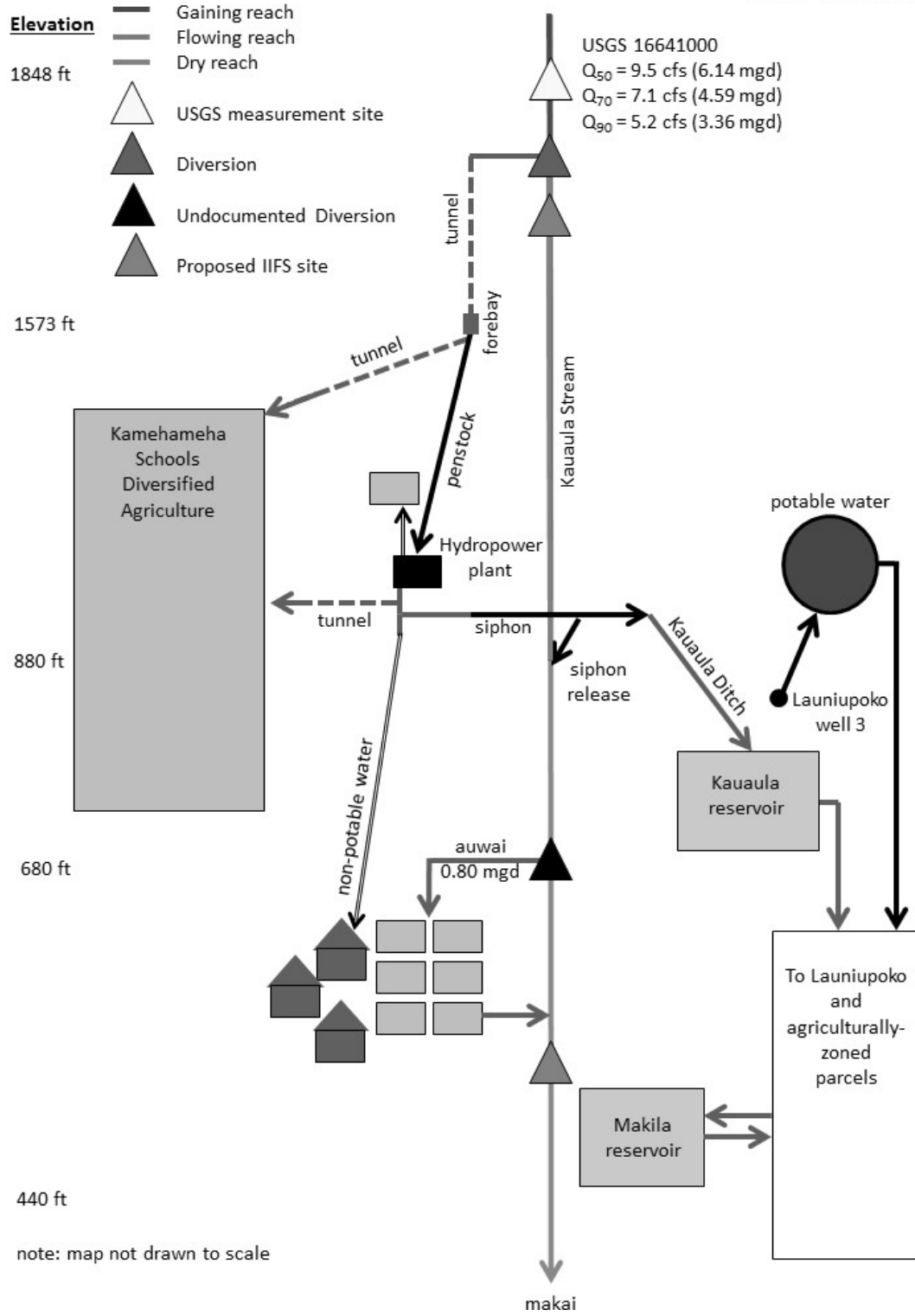
Figure 10: Simplified schematic diagram for the hydrologic unit of Kaua'ula (6007).
