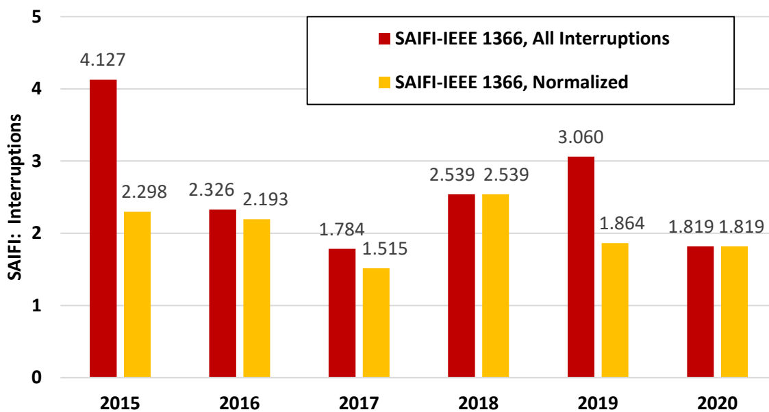
Figure 10 – HELCO System Average Interruption Frequency Index (Generation, Transmission, and Distribution events)
