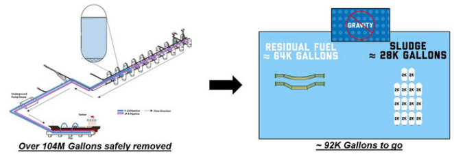
Fuel Remaining Following Gravity Defueling
